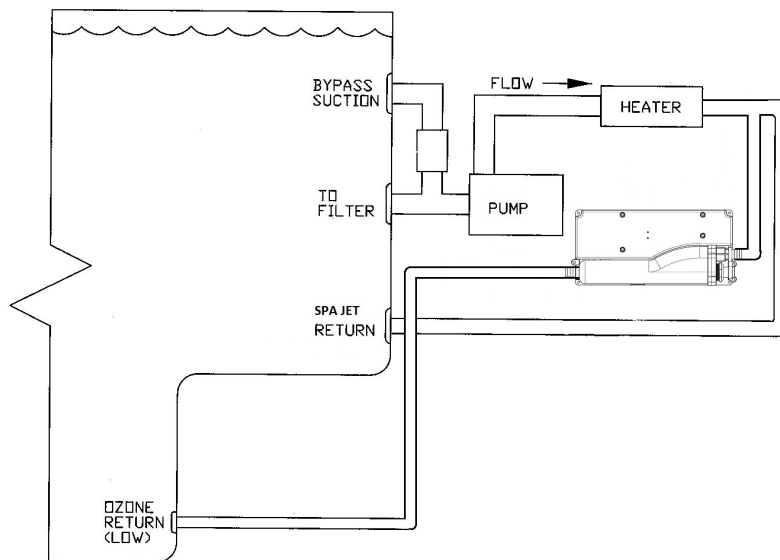
By-Pass (Side-stream) Plumbing Schematic
